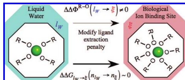
Figure 3. Schematic illustrating the general idea that when an ion is transferred from one environment (say liquid water l_w ) to another (say biological ion-binding site \xi ), then the free energy cost \Delta\Delta G_{l_w \rightarrow \xi}(n_{l_w} \rightarrow n_{\xi}) associated with changes in the coordination number of the ion ( n_{l_w} \rightarrow n_{\xi} ) can be overcome through modifications in free energy penalties \Delta\Delta\Phi^{R-O}(l_w \rightarrow \xi) associated with extracting ligands from their environments.
