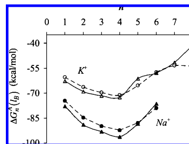
Figure 4. Solvation free energies of \Delta G_n^A(l_B) of ions A \in \{\text{Na}^+, \text{K}^+\} in liquid formamide ( l_B = l_{\text{formamide}} ; triangles connected using solid lines) and liquid methanol ( l_B = l_{\text{methanol}} ; circles connected using broken lines) estimated using the quasi-chemical framework.
