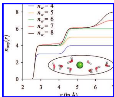
Figure 5. Number distributions n_{\text{oxy}}(r) of water oxygens around \text{K}^+ . Each curve represents an individual simulation in which the natural partial charges of only a subset of randomly selected water molecules n_w in the simulation box are turned on, while the natural partial charges on the remaining water molecules in the simulation box are turned off. The inset illustrates a representative configuration when the partial charges on exactly n_w = 8 water molecules are turned on.
