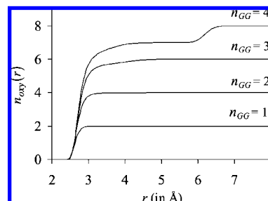
Figure 6. Number distributions n_{\text{oxy}}(r) of the oxygens belonging to the glycine dipeptide ( GG ) molecules around \text{K}^+ . Each curve represents an individual simulation in which n_{GG} glycine dipeptide molecules are present in the simulation box. Note that glycine dipeptide molecules are bidentate ligands, and in contrast to water molecules, provide two oxygen ligands for ion coordination.
